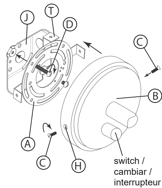
DRAWING 1 - MOUNTING
