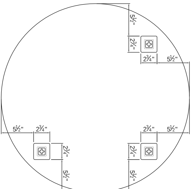
Back view
