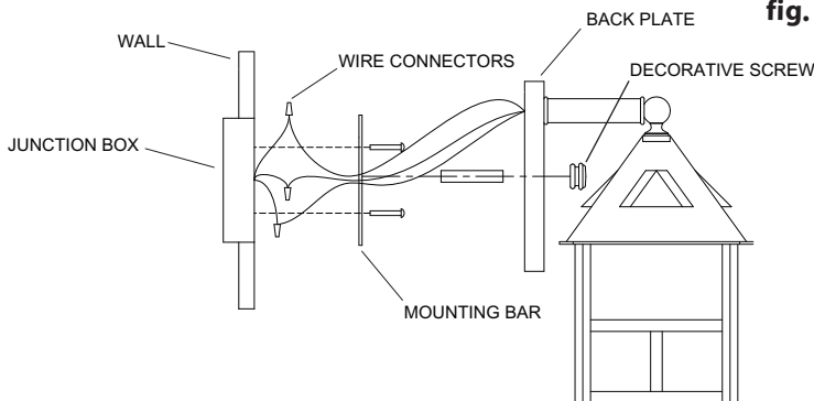
Wall Mount fig. C
